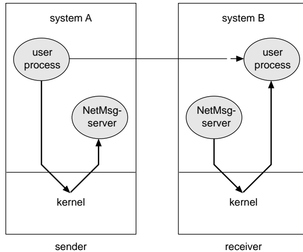
Figure A.7 Network IPC forwarding by NetMsgServer.
