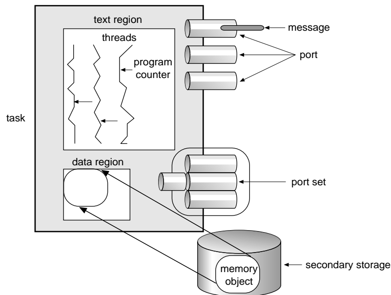
Figure A.2 Mach's basic abstractions.
