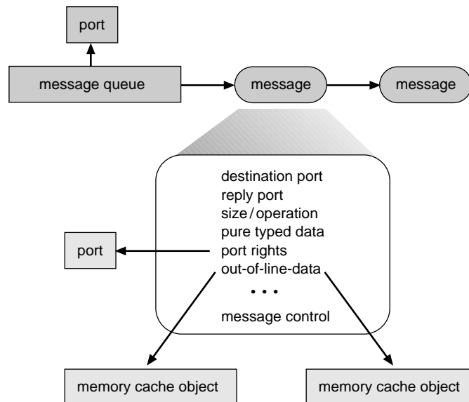
Figure A.5 Mach messages.
