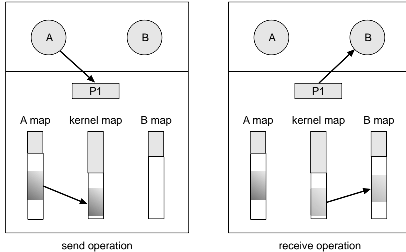
Figure A.6 Mach message transfer.
