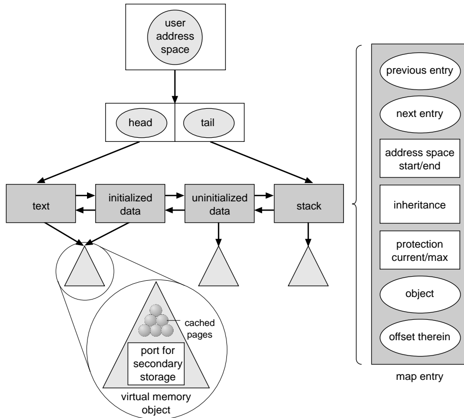
Figure A.8 Mach virtual memory task address map.
