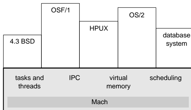
Figure A.1 Mach 3 structure.
